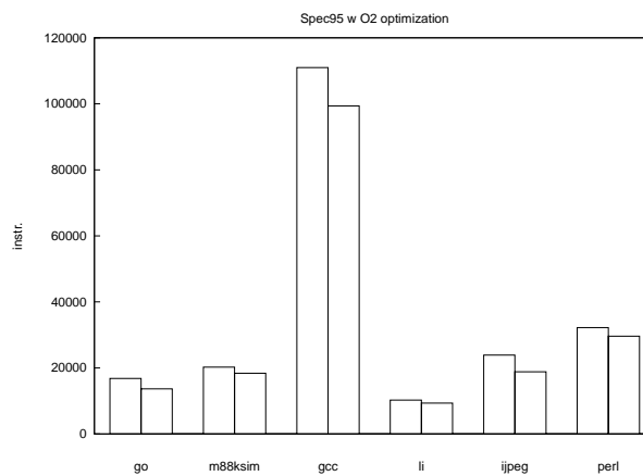
Figure 10: Results for level O2 optimized assembly code
