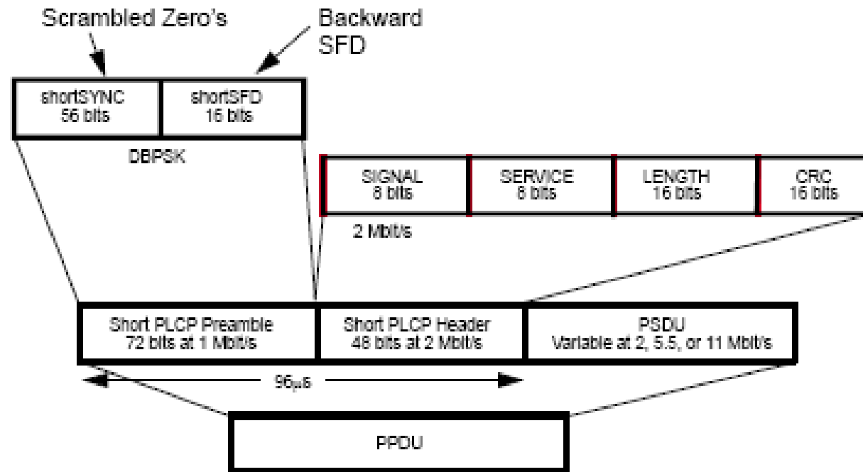
Figure 128 – Short PLCP PDU format
