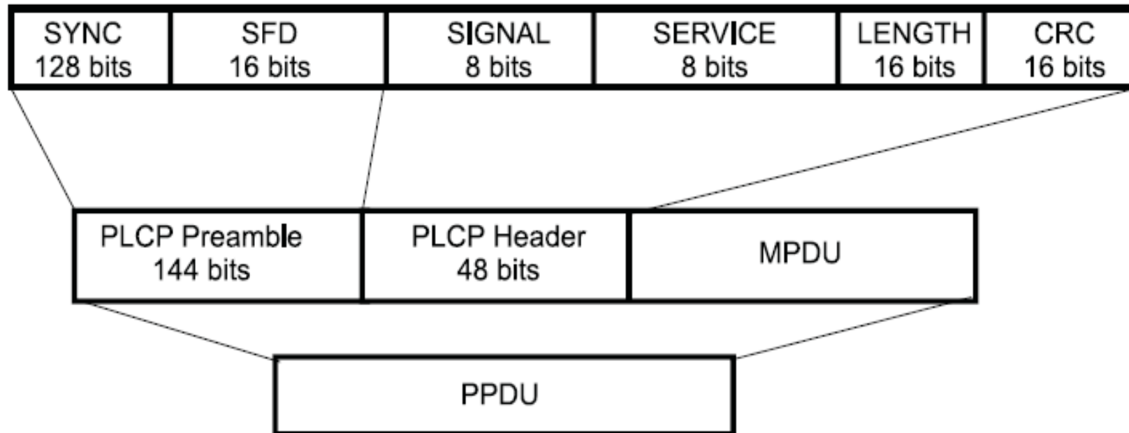
Figure 86—PLCP frame format
