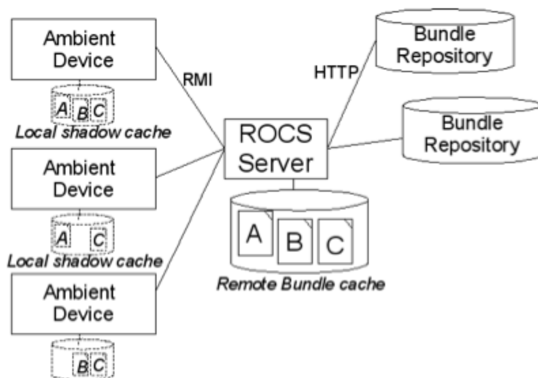
Figure 1: ROCS Architecture
